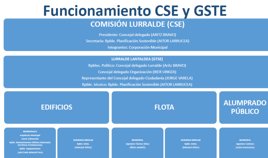
Figura 1. Organigrama CSE
